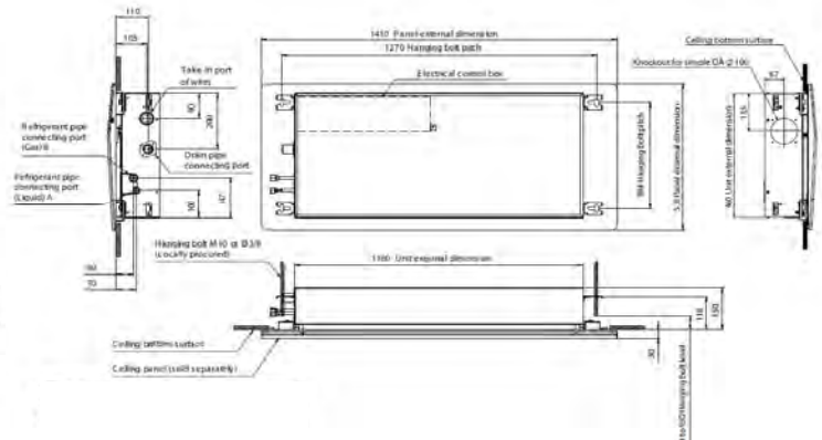
40VU0151-8S-TST to 40VU0271-8S-TST
