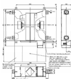
VN-U00151SY-E to VN-U00251SY-E
