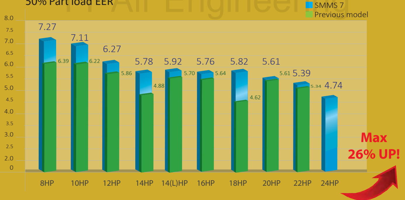
50% Part load EER
