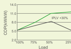
Part Load Efficiency(AHRI)
