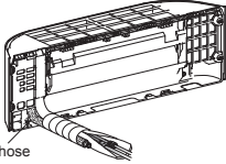
Drain hose
