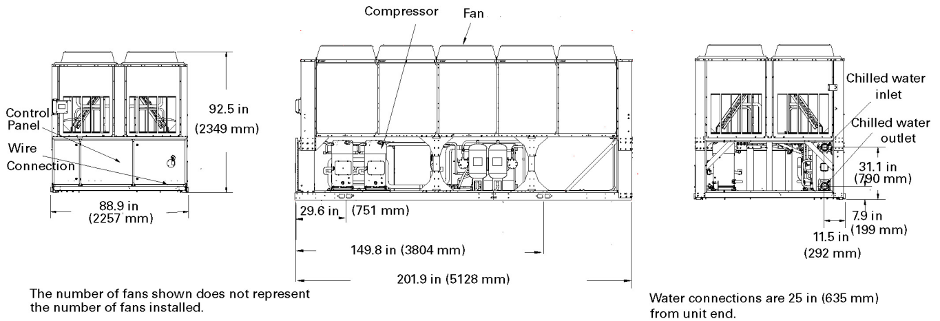
Figure 13. CGAM 110 and 120 (comprehensive acoustic package versions), 140 (compact version), CXAM 90 (comprehensive acoustic package versions), 100 (compact and comprehensive acoustic package versions), 110 and 120 (compact version)
